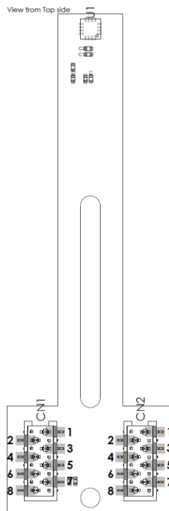
Figure 47: LT Type 5 Connector Pinout
