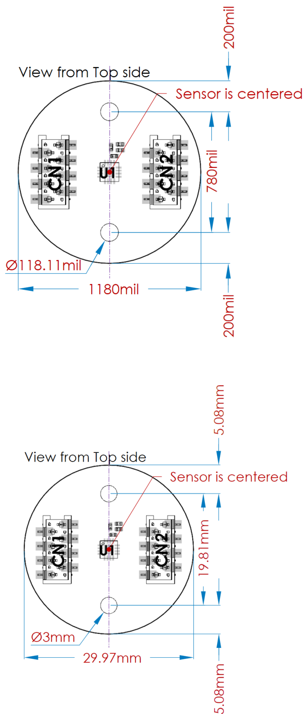
Figure 26: RD Type 3 Mechanical Drawing
