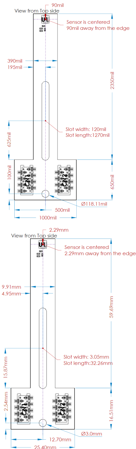
Figure 27: LT Type 3 Mechanical Drawing, mil = 0.001" = 0.0254mm
