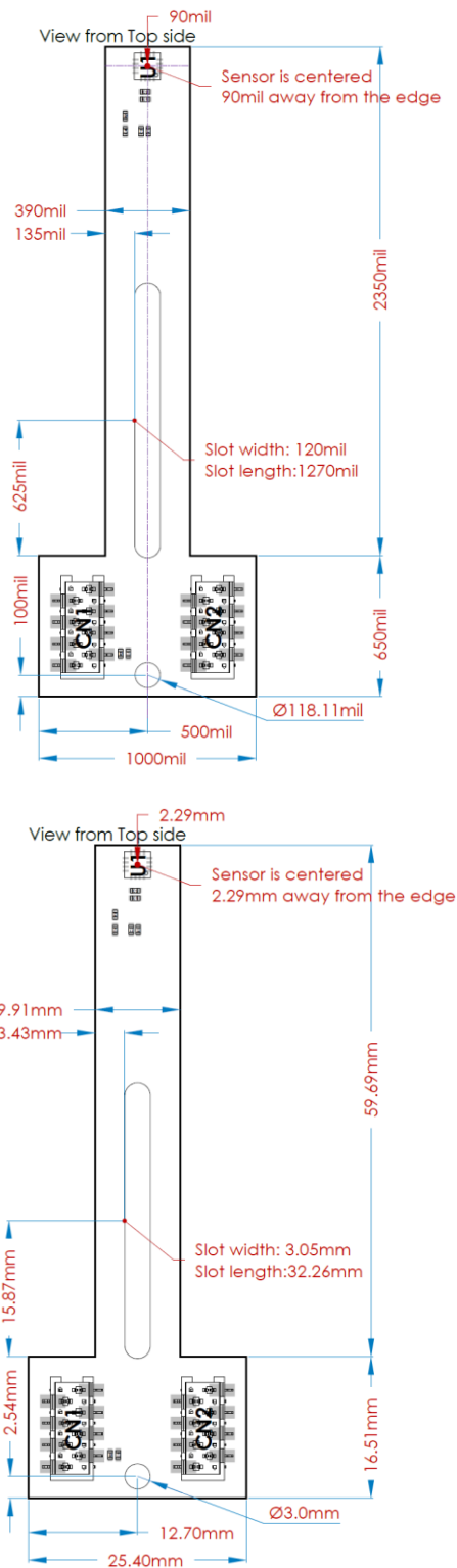
Figure 45: LT Type 5 Mechanical Drawing, mil = 0.001" = 0.0254mm
