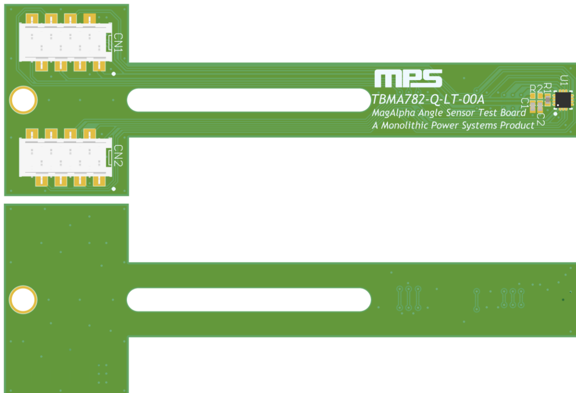
Figure 31: LT Type 4 Board Overview
