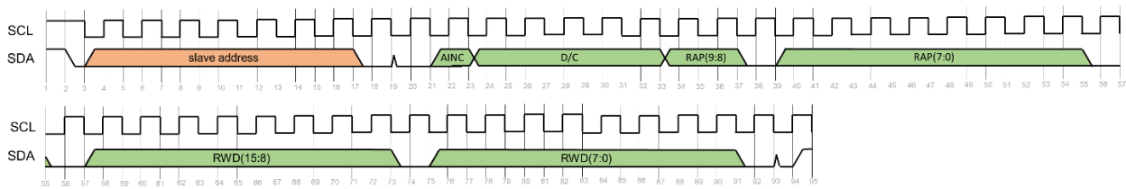
Figure 10. I2C write cycle
