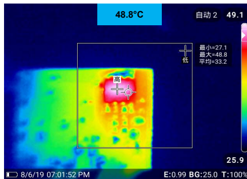
Thermal V_{IN}=265V_{AC}
