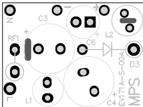
Figure 2: Top Layer
