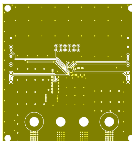
Figure 4: Inner Layer 2
