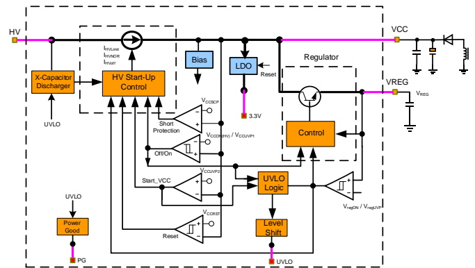
Figure 3: Power Supply Block Diagram
