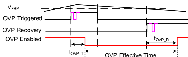
Figure 14: Output OVP
