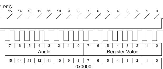
Figure 13: Write Register Operation with Two 16-Bit Frames
