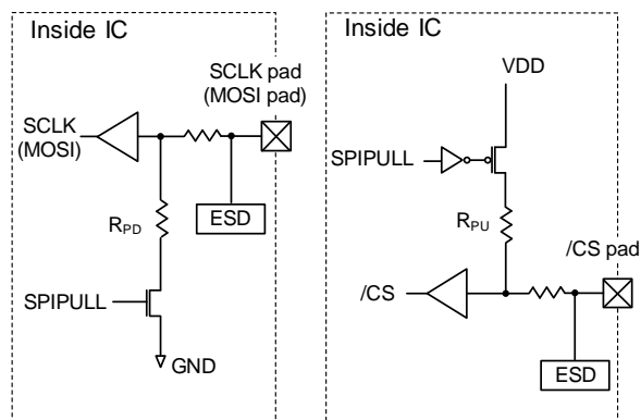
Figure 28: SPI Input Pins Circuit in the IC
