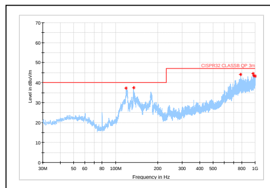
Radiated Emissions 30MHz to 1GHz, CISPR32 Class B (8)
