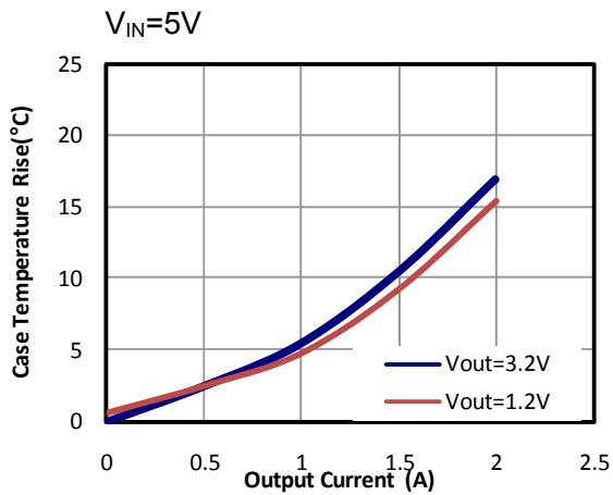
Case Temperature Rise vs. Output Current
