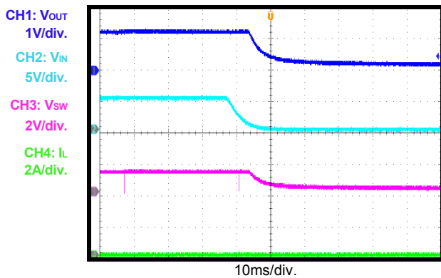
V_{IN} Shutdown
