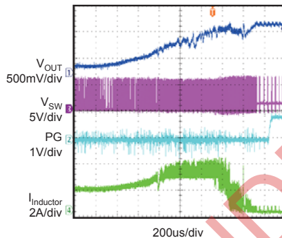
Short Recovery for ASYN Mode V_{OUT} = 0.9V , I_{OUT} = 50mA
