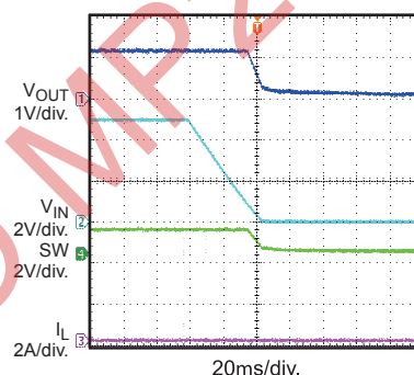
V_{IN} Shut down without Load
