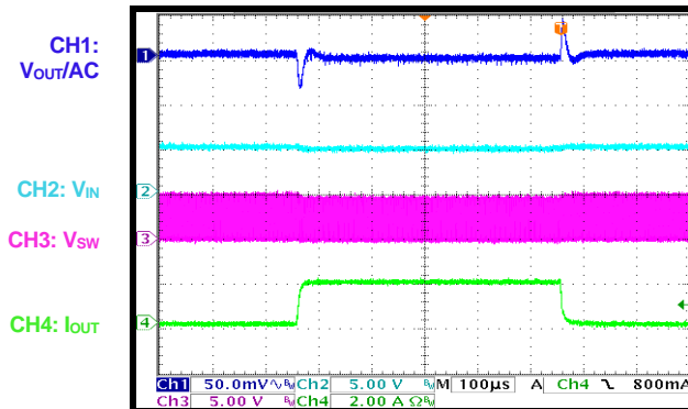
Load Transient V_{IN} = 5V , I_{OUT} = 0A to 2A
