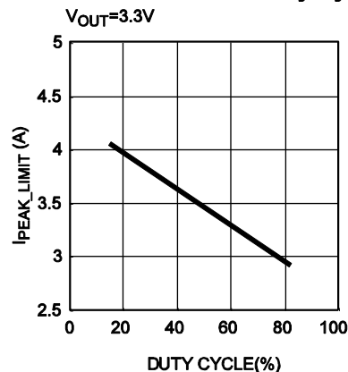
Current Limit vs. Duty Cycle
