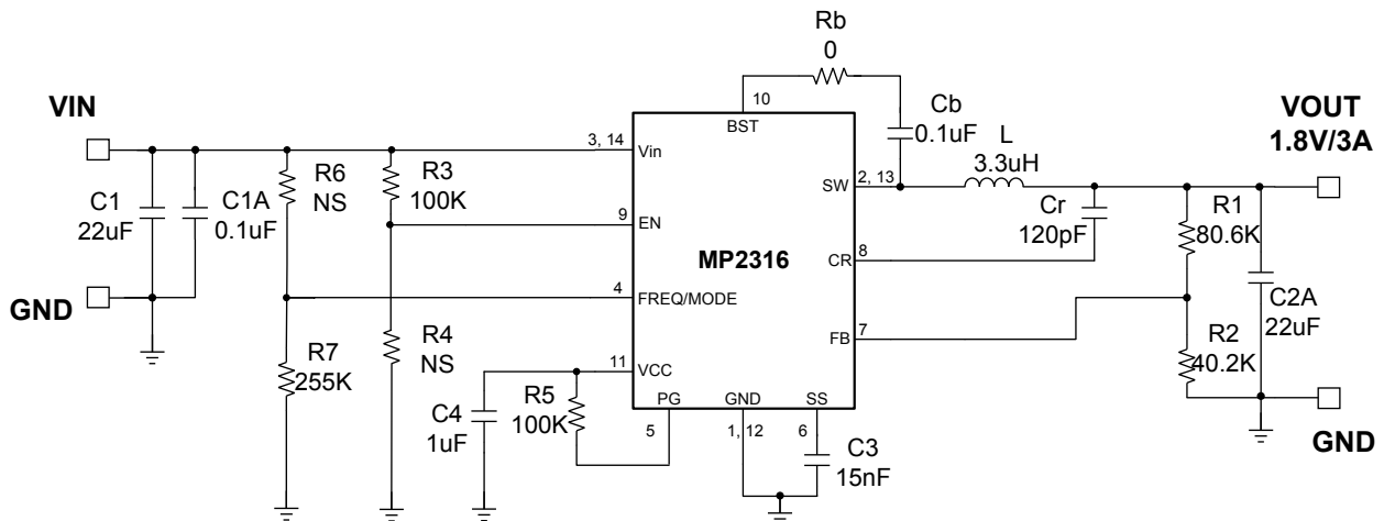
Figure 18— V_{IN}=12V , V_{OUT}=1.5V , I_{OUT}=3A , F_S=500kHz
