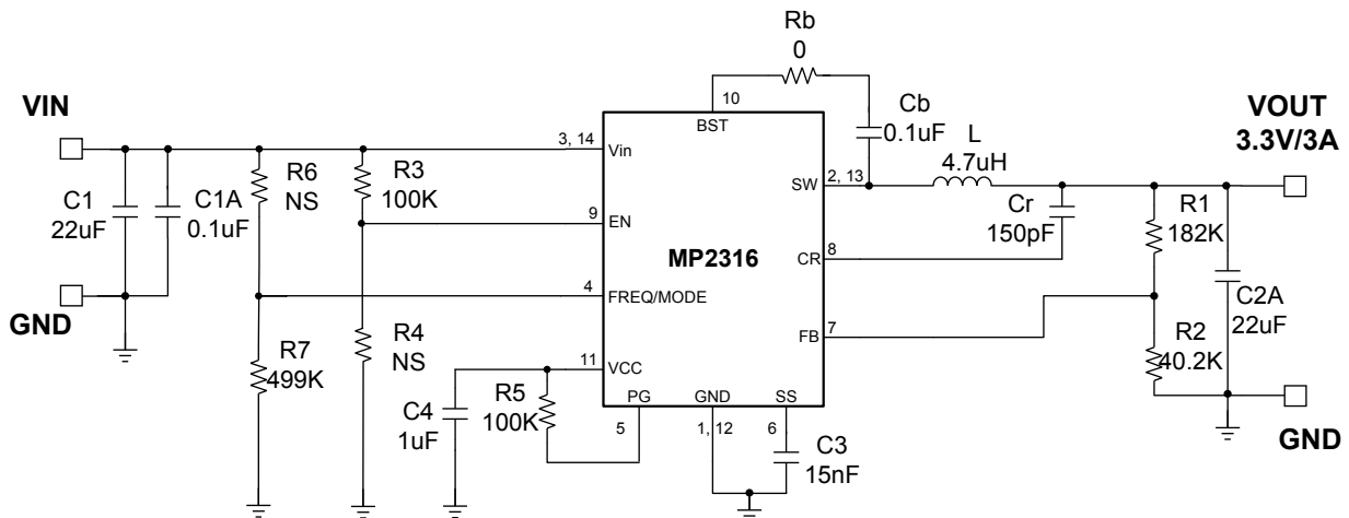
Figure 20— V_{IN}=12V , V_{OUT}=2.5V , I_{OUT}=3A , F_S=500kHz
