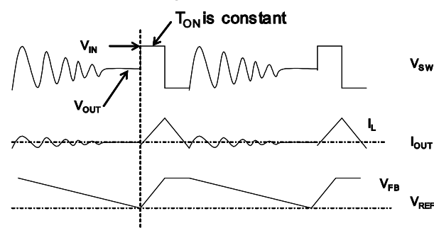
Figure 3: Light-Load Operation
