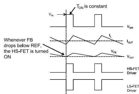
Figure 2: Heavy-Load Operation
