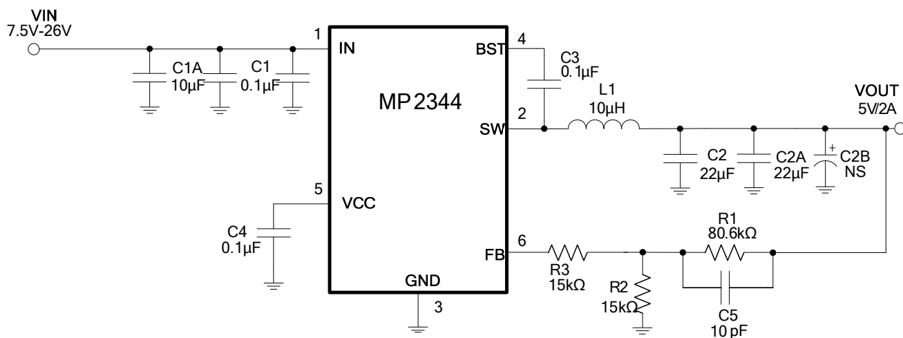
Figure 7: 5V/2A Output
