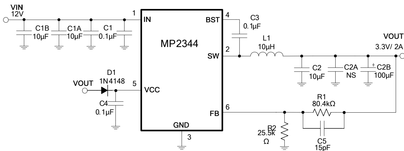
Figure 8: 3.3V/2A Output
