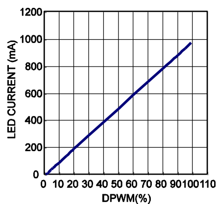
PWM Dimming
