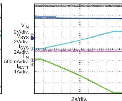
System Current Transient
