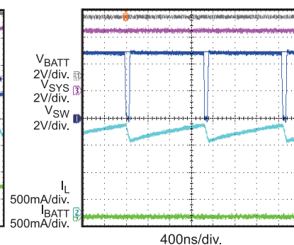
Input Current Limit
