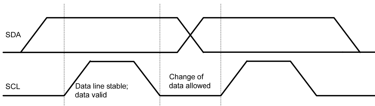
Figure 16: Bit Transfer on the I 2 C Bus
