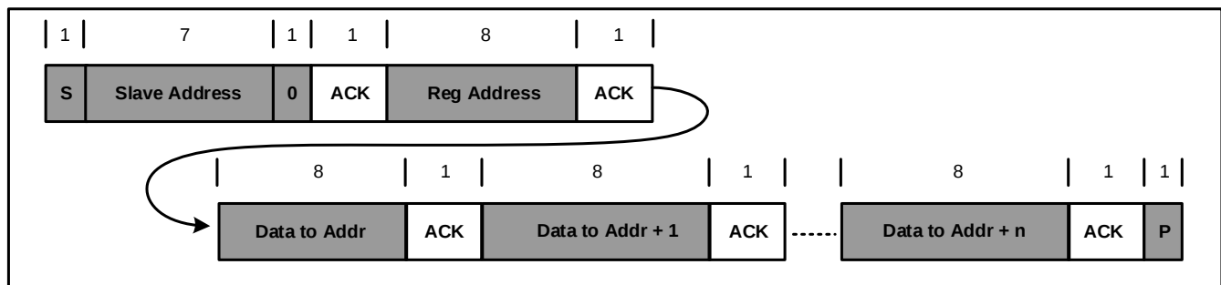
Figure 13: Multi-Write Sequence
