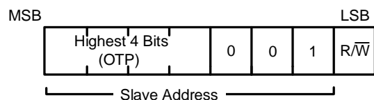
OTP Address
