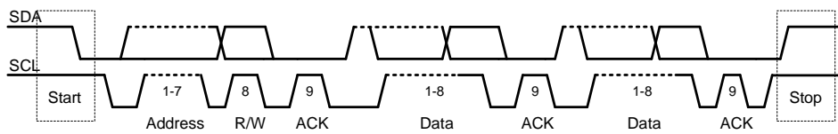
Figure 16: Byte Format
