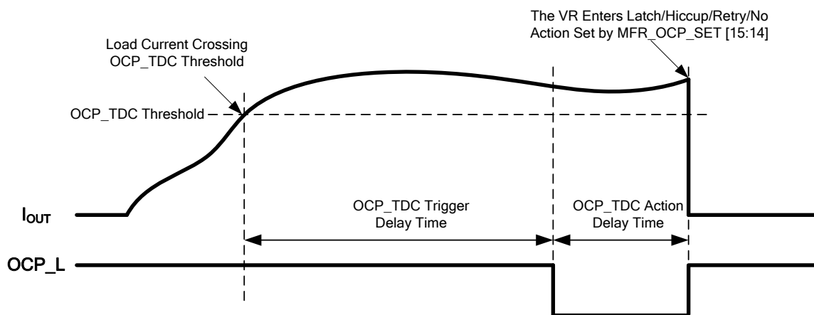
Figure 25: OCP_TDC Action
