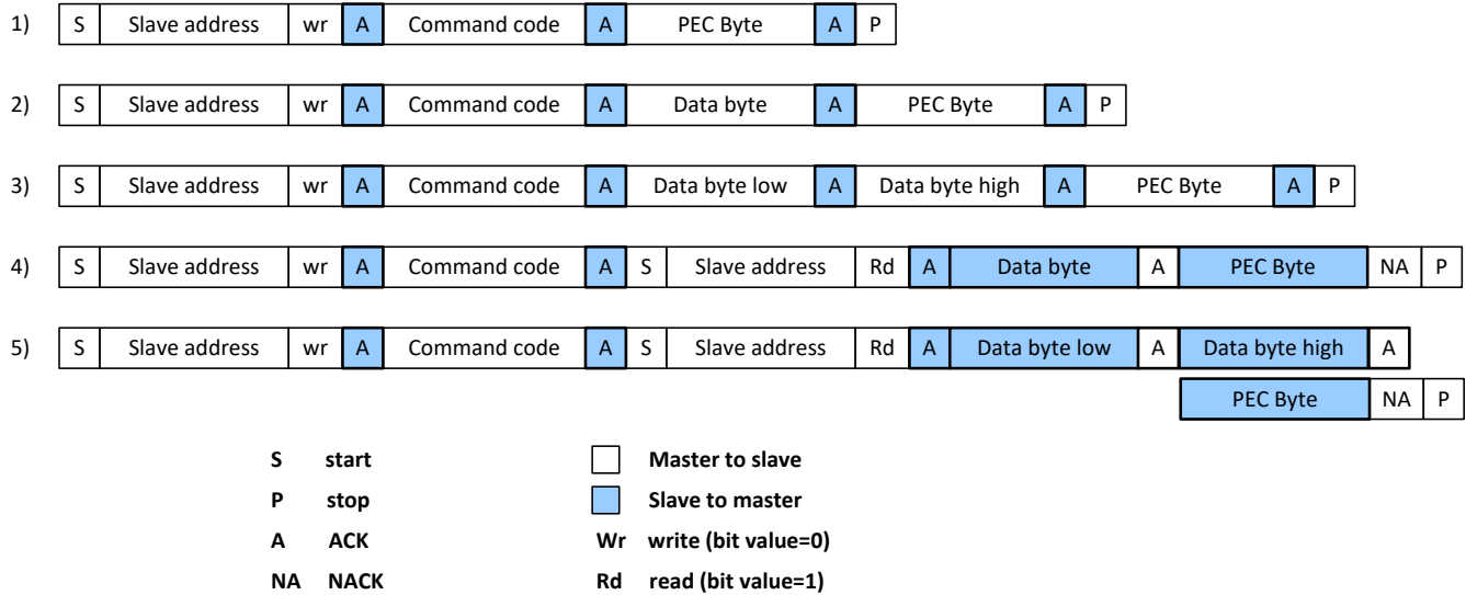
Figure 20b: Supported PMBus/I²C Transmission Structure with PEC
