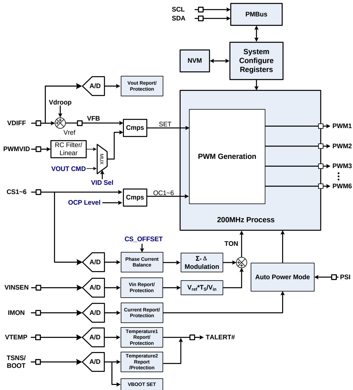
Figure 1: System Functional Block
