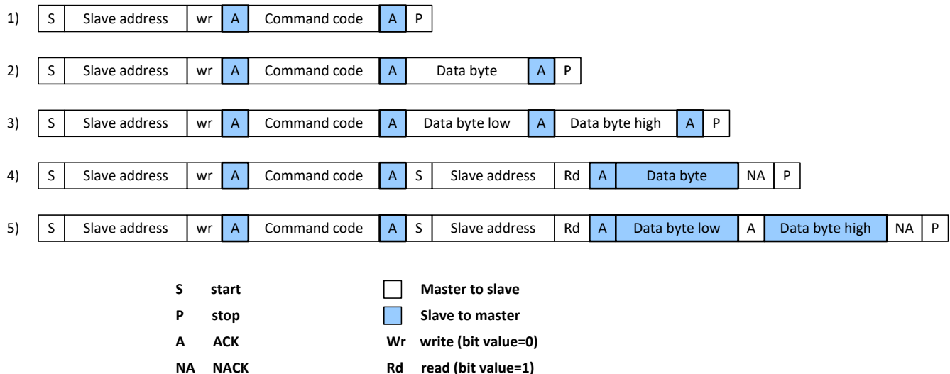
Figure 20a: Supported PMBus/I 2 C Transmission Structure without PEC
