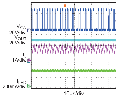
Mix Dimming by I 2 C Interface D_{DIM} = 60\%
