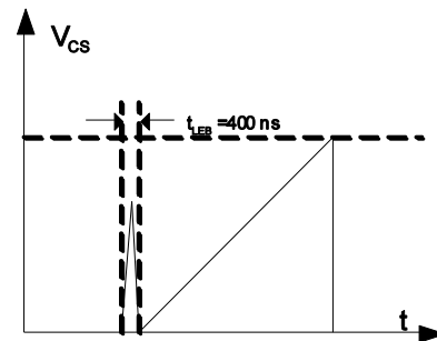
Figure 6: Leading-Edge Blanking
