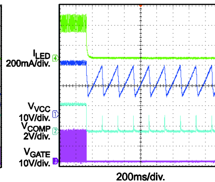
Primary-Side OCP Protection
