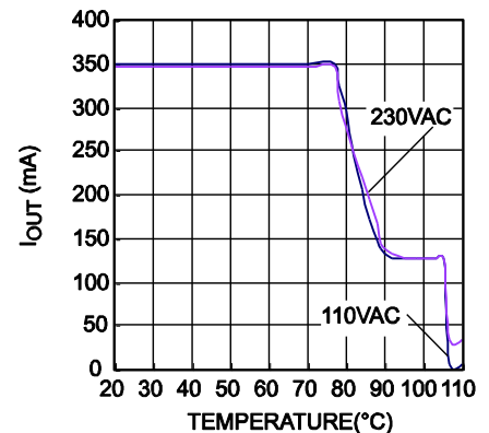
NTC Curve
