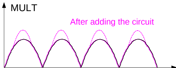
Figure 15: The MULT Signal with THD Improved Circuitry
