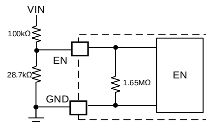
Figure 5: EN Connection
