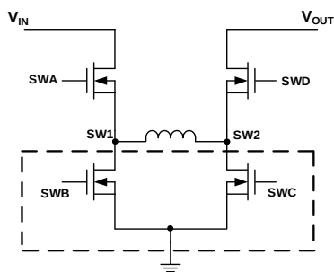
Figure 3: Buck-Boost Topology
