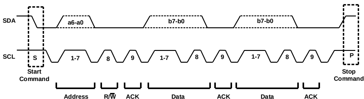
Figure 8: Data Transfer over the PMBus
