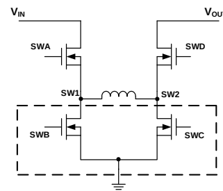
Figure 13: Buck-Boost Topology
