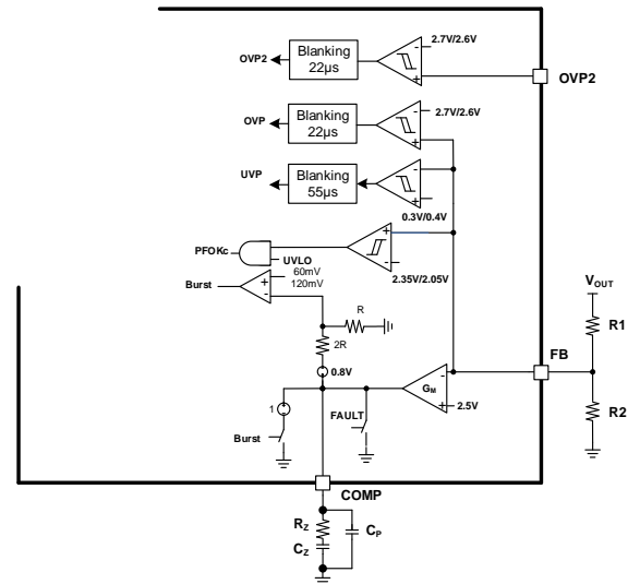
Figure 13: FB Functional Block
