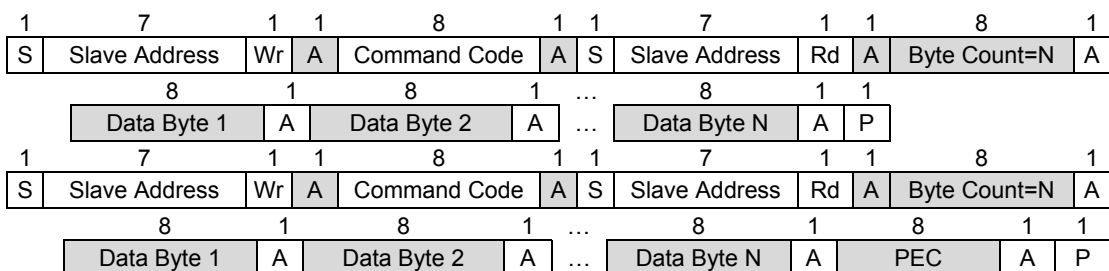
Figure 15: PMBus™ Message Format
