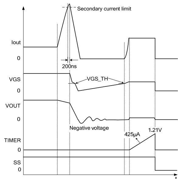
Figure 2: SCP in Latch-Off Mode
