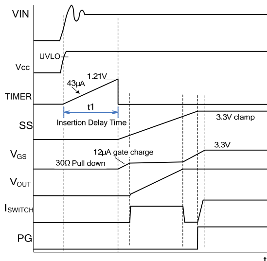
Figure 5: Start-Up Sequence
