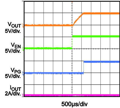
EN Startup (Load Switch)
