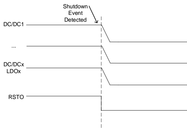
Figure 6: Shutdown Sequence
