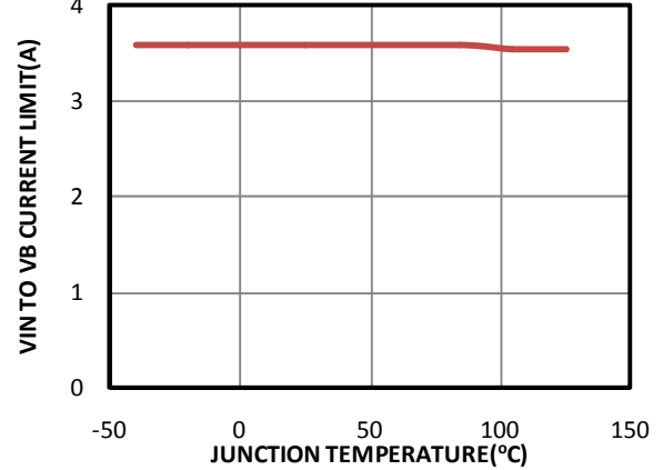
V_{IN} to VB Current Limit vs. Temperature Rlimit=1.4k
