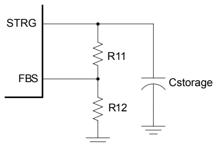
Figure 5. Storage Feedback Circuit
