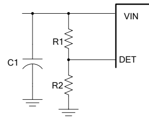
Figure 14: Release-Feedback Circuit
