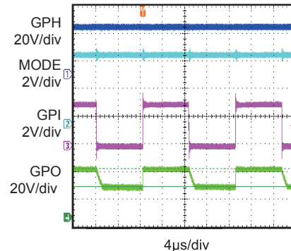
Gate Pulse Management MODE1
