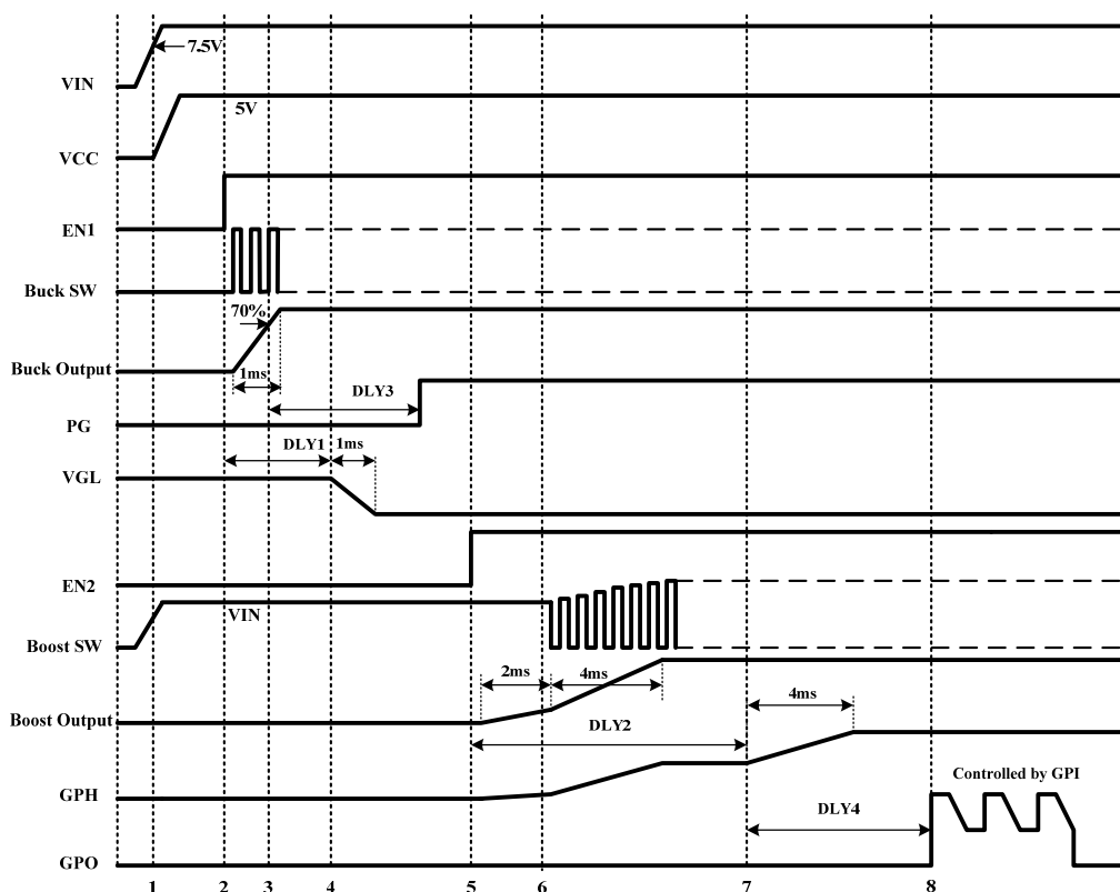
Figure 9—Power-On Sequence
