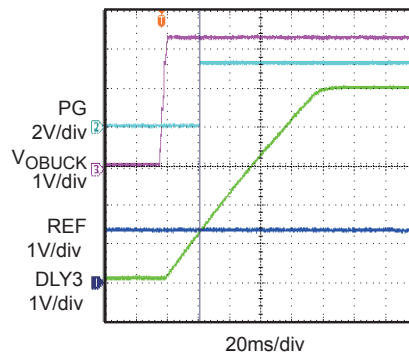
Buck Regulator Power Good Signal
