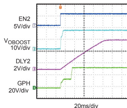
Power On Sequence
