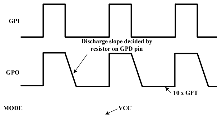
Figure 7 Gate Pulse Management at Mode 1
