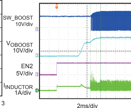
Boost Regulator EN2 Start Up
