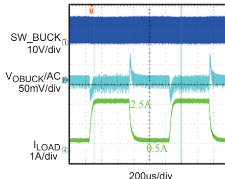
Buck Regulator Load Transient
