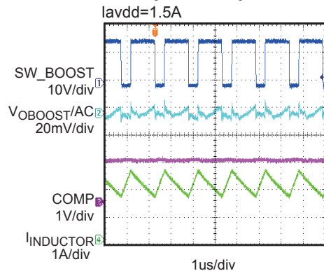
Boost Regulator Steady State Operation
