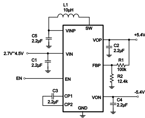
Figure 2: Application Circuit
