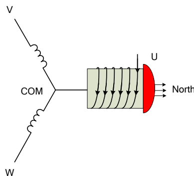
Figure 7: Magnetic North with Winding Direction
