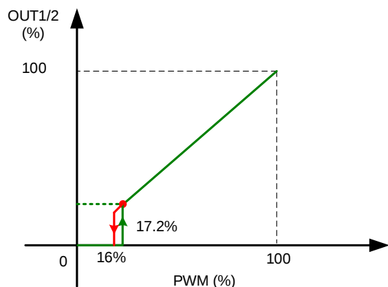
Figure 2: Minimum Input PWM Duty
