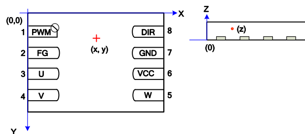
Figure 3: Hall Position
