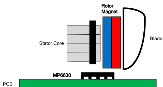
Figure 5: The MP6630 on the Top of the PCB (Side View)
