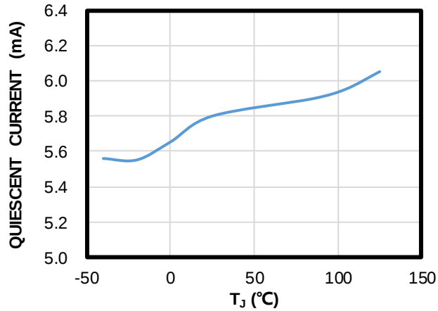
Quiescent Current vs. T_J
