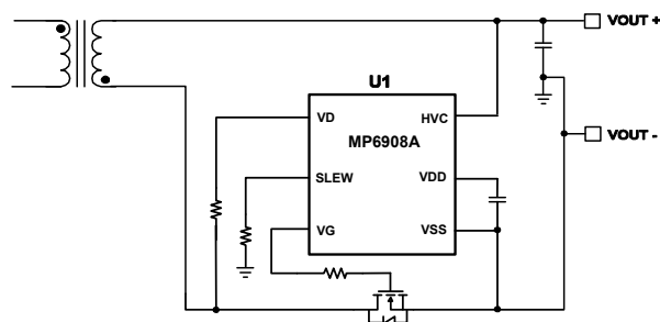
Figure 5: Low-Side Rectification
