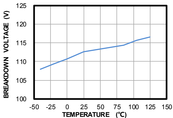
VD-VS Breakdown Voltage vs. Temperature
