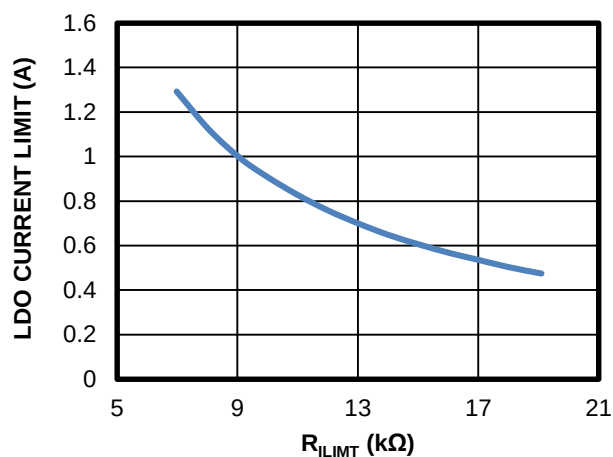
LDO Current Limit vs. R ILIMIT
