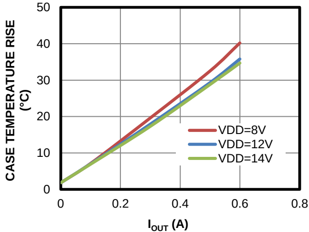
Boost Mode Plot
