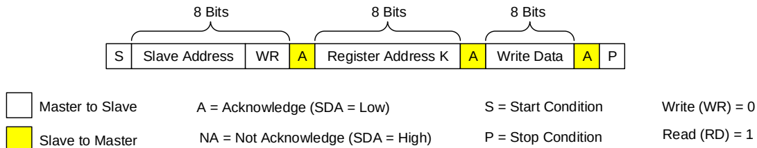
Figure 11: I 2 C Write Example
