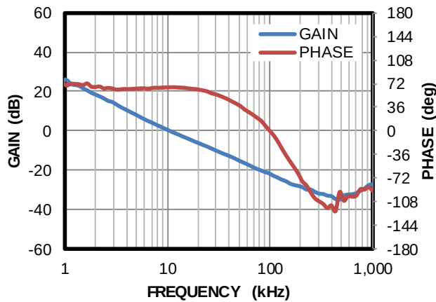
Boost Mode Plot
