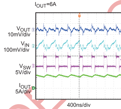
Steady State I_{OUT}=6A
