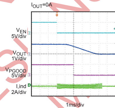
PGOOD, Shutdown Through EN I_{OUT}=0A
