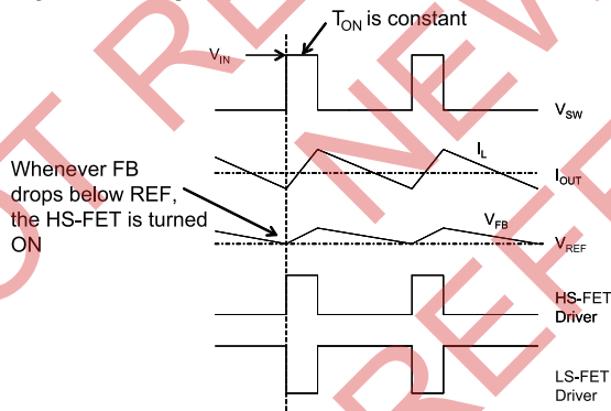
Figure 2: Heavy-Load Operation
