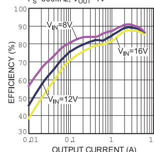
Efficiency vs. Output Current F_S=500\text{kHz} , V_{OUT}=1\text{V}
