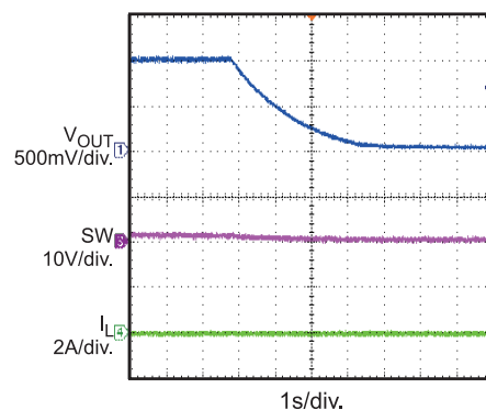
Thermal Shutdown
