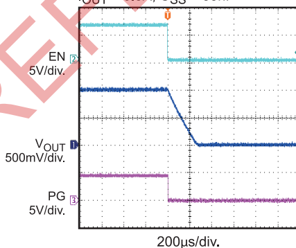
Power Good through EN Shutown
