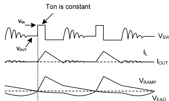
Figure 4: Light-Load Operation
