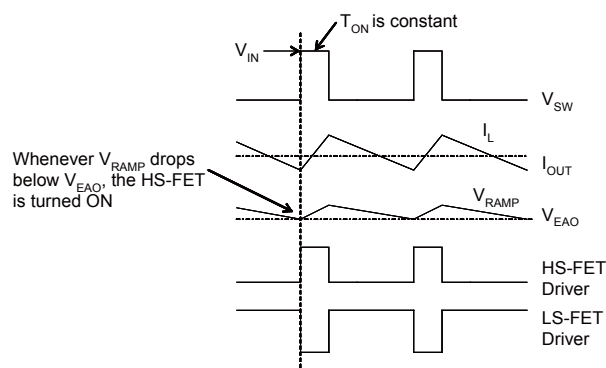
Figure 3: Heavy-Load Operation
