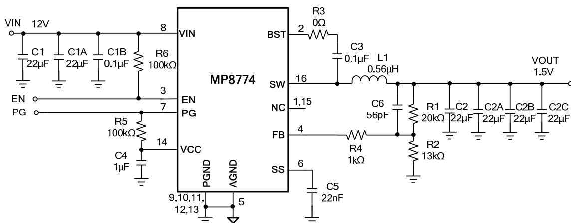
Figure 11: V_{IN} = 12V , V_{OUT} = 1.5V , I_{OUT} = 12A (8)
