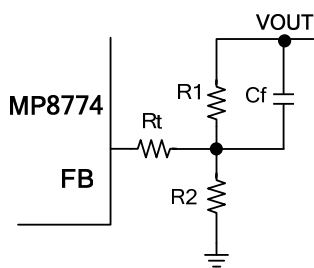
Figure 7: Feedback Network
