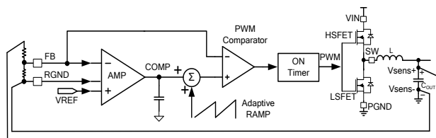
Figure 2: COT Control
