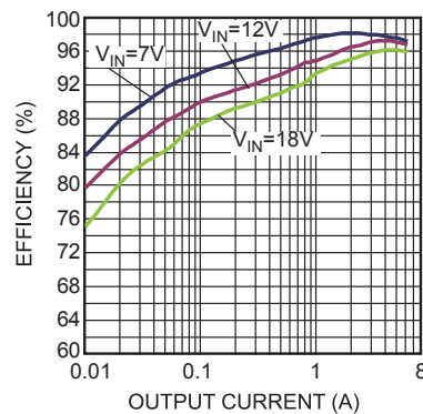
Efficiency vs. Output Current V_{OUT}=5V , L=3.3\mu H , DCR=4.4m\Omega
