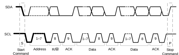
Figure 12: Complete Data Transfer
