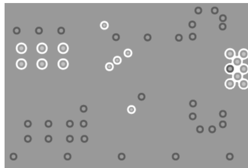
Mid-Layer 1
