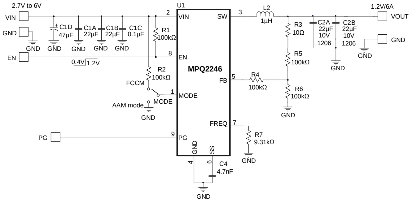
Figure 6: V_{OUT} = 1.2V , I_{OUT} = 6A Application Circuit
