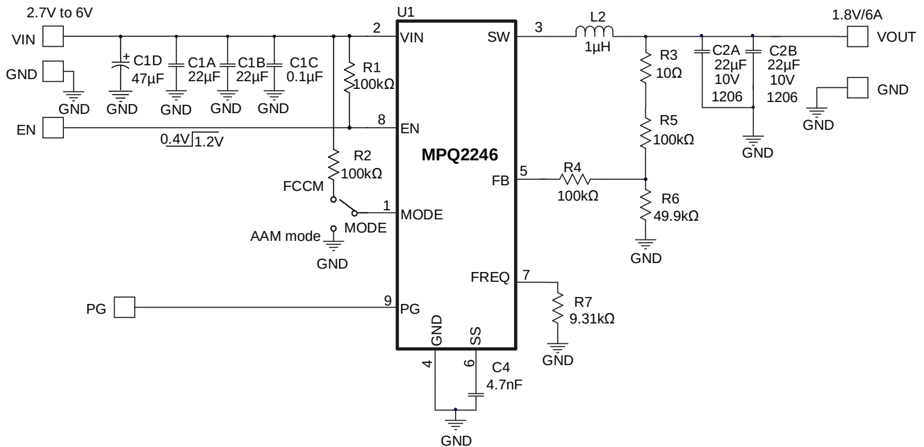
Figure 5: Typical Application Circuit ( V_{OUT} = 1.8V , I_{OUT} = 6A )
