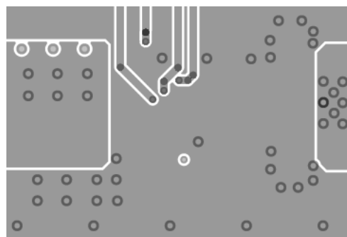
Mid-Layer 2
