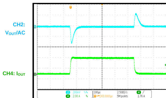
Load Transient
