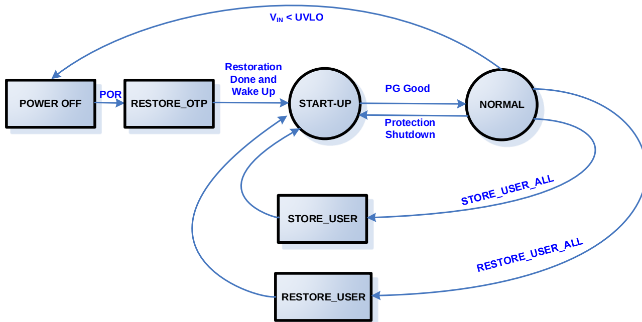
Figure 10: System State Machine
