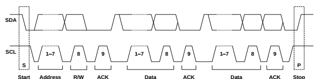
Figure 7: A Complete Data Transfer
