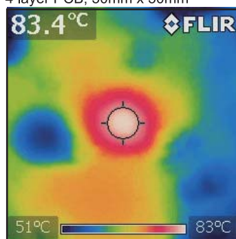
Thermal Image
