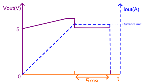
Figure 7: Over-Current Limit
