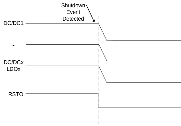
Figure 6: Shutdown Sequence
