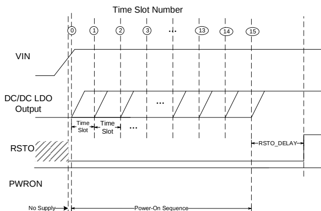
Figure 4: Power-On Sequence
