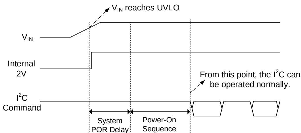
Figure 11: I 2 C Timing Graph
