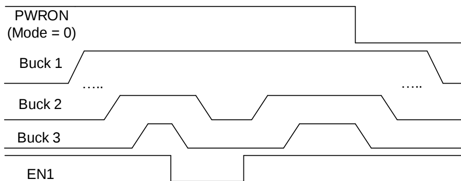
Figure 10: EN1 Function
